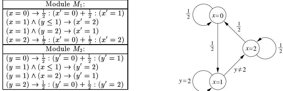
Fig. 2. (i) A system composed of two modules. (ii) Transition system of module M_1
