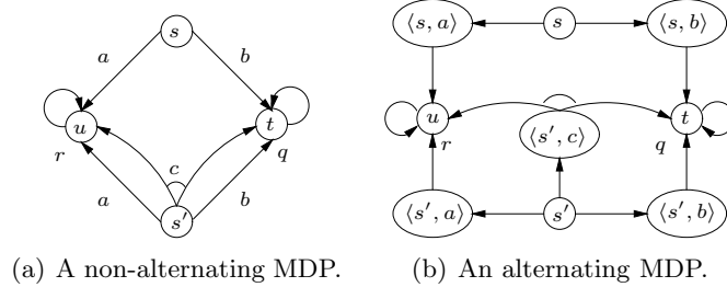
Figure 7: MDPs illustrating how separating nondeterministic and probabilistic choice does not help to compute \approx^{>0} .
