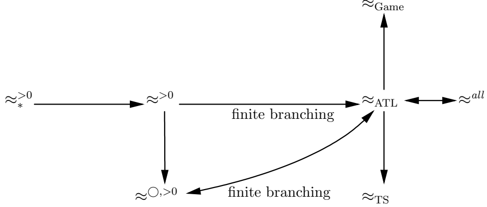
Figure 3: Relationship between equivalence relations for MDPs.
