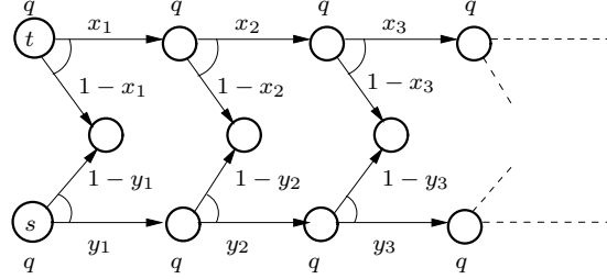
Figure 6: An infinite Markov chain on which \approx_{\text{ATL}} \not\subseteq \approx^{>0} , where x_i 's and y_i 's represent the probabilities that the corresponding edge is taken.
