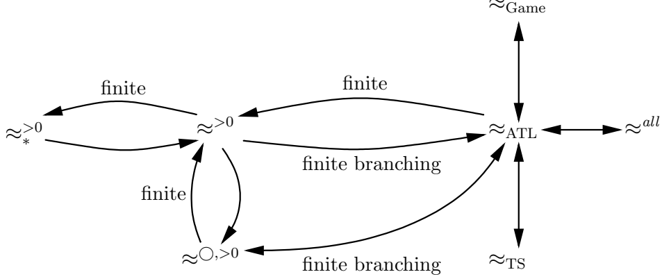
Figure 2: Relationship between equivalence relations for AMDPs.
