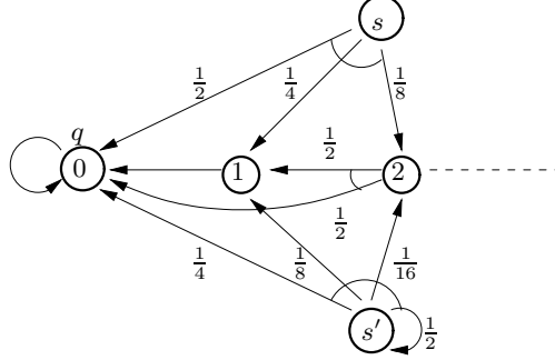
Figure 4: An infinite Markov chain in which states s and s' cannot be distinguished by \text{QRCTL}^{>0} , but are distinguished by the ATL formula \langle\langle p \rangle\rangle \Box \neg q .
