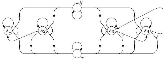
Figure 8: MDP showing the lack of 1-neighbourhood refinement operators.
