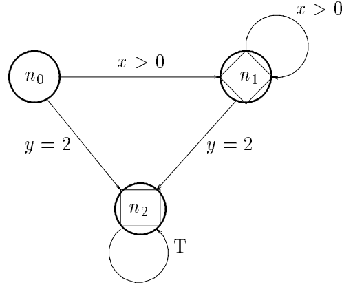
Figure 5: Automaton for (x > 0) \mathcal{W} (y = 2) .
