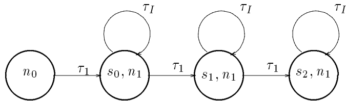
Figure 7: Behavior automaton.
