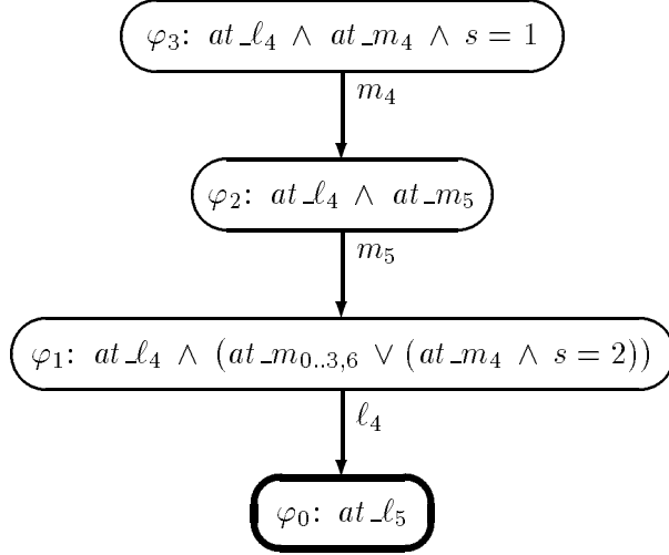
Figure 3: Verification diagram for 1-bounded overtaking.
