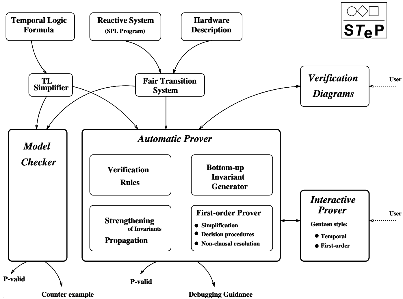
Figure 1: An overview of the STeP system
