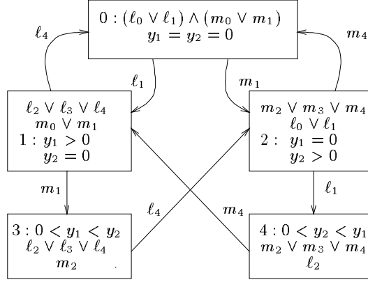
Fig. 2. Verification diagram A_0 for property \square \neg(\ell_3 \wedge m_3) of BAKERY.
