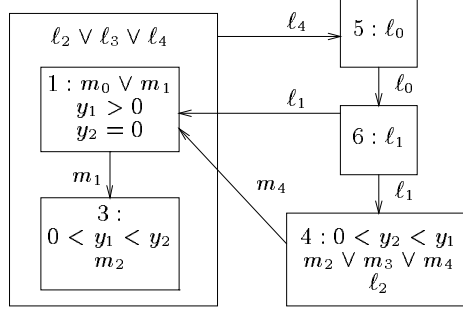
Fig. 3. Fairness diagram A_1 , obtained from Figure 2.
