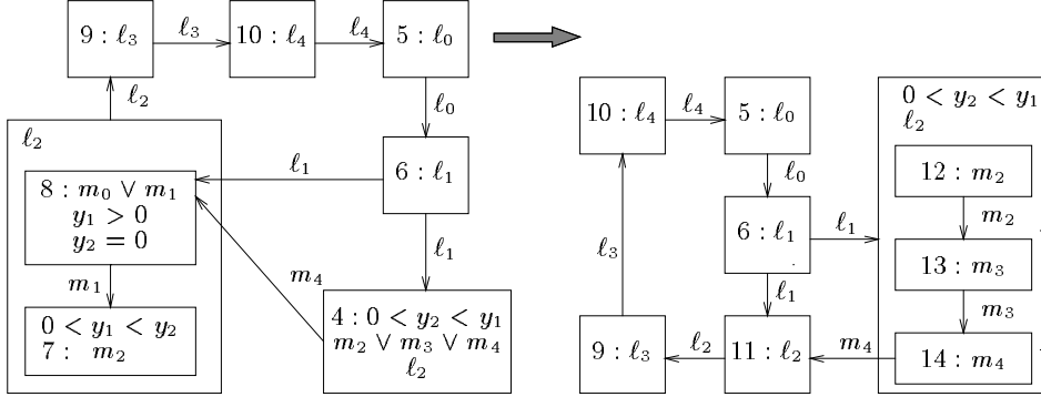
Fig. 4. Fairness diagrams A_2 and A_3 , proving accessibility of BAKERY.
